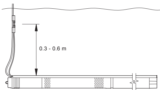
Fig. 3 Horizontal installation
