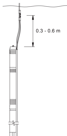
Fig. 2 Vertical installation
